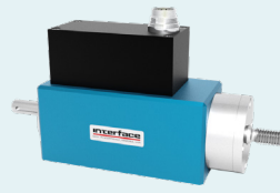
AT104 Compact Size Force and Torque 4.5/0.89 lbf/lbf-in and 11.2/4.4 lbf/lbf-in 20/0.1 N/Nm and 50/0.5 N/Nm
