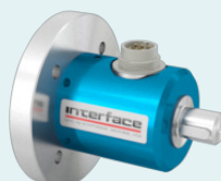
TS18 Shaft to Flange Style 44.3 lbf-in to 17.7K lbf-in 5 Nm to 2K Nm
