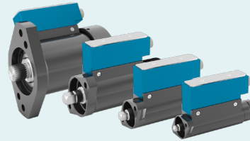
T31, T32, T33, & T34 Spindle Torque 8.85 lbf-in to 4.43K lbf-in 1 Nm to 500 Nm
