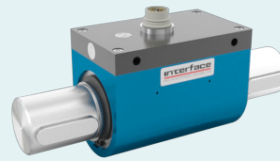
T14 Slip-Ring 8.85 lbf-in to 4.43K lbf-in 1 Nm to 500 Nm
