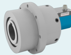
T22 Pulley Belt 177 lbf-in to 44K lbf-in 20 Nm to 5K Nm
