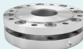
TS19 Short Flange Style 443 lbf-in to 88.5K lbf-in 50 Nm to 10K Nm
